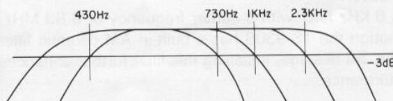
Fig.-53 SP-930 filter characteristics
