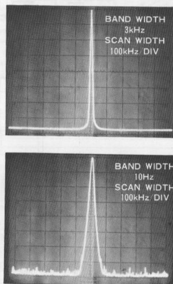
Fig.-7 VCO C/N characteristic
