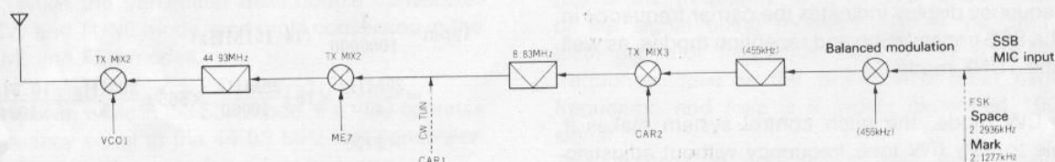
Fig.-4 Transmitter frequency configuration block diagram
