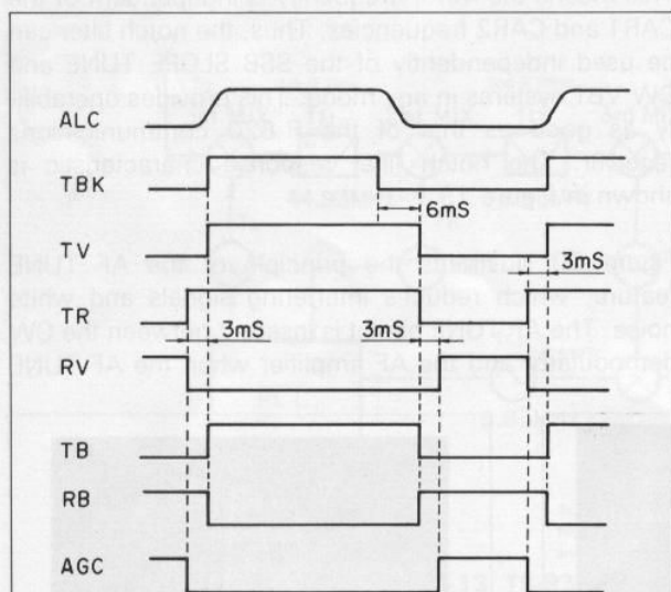
Fig.-21 Timing chart for transmit/receive's signals in the SSB, FSK, TUNE or CW full break-in modes
