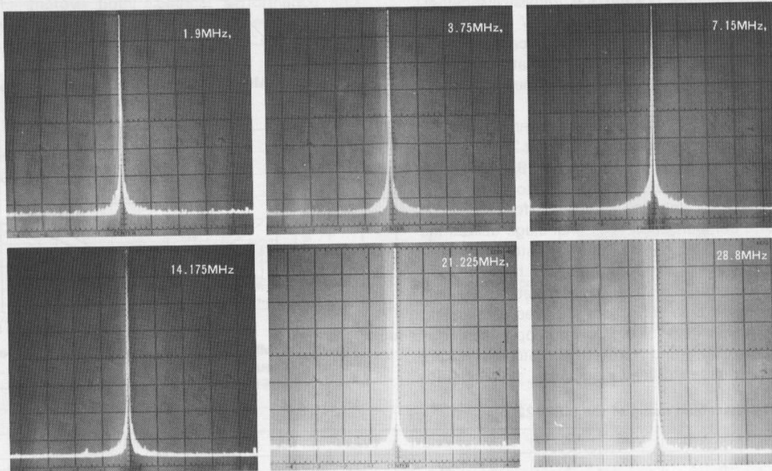
Fig.-43 Adjacent spurious radiation (BW 1 kHz SW 100 kHz/DIV)
