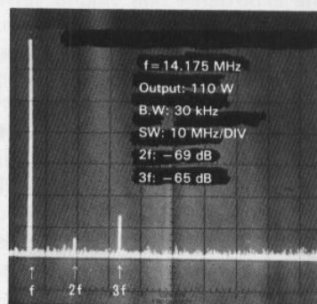
Fig.-46 The harmonic and spurious signal output
