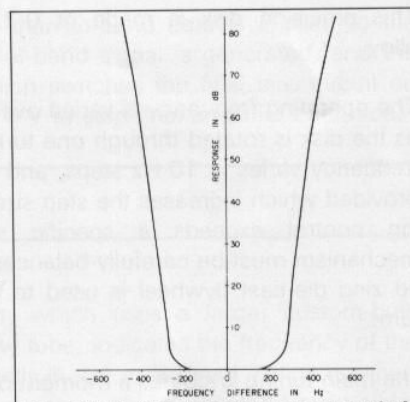
Fig.-52(d) YG-455CN-1 characteristic
